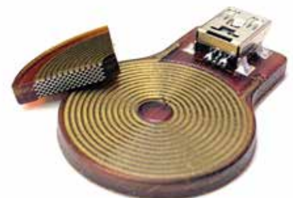
Inductor coil
